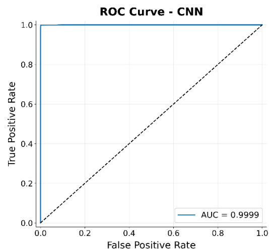
Test ROC Curve for the CNN Model
