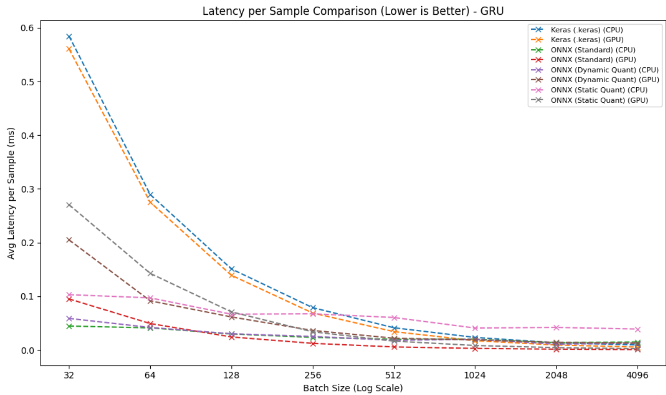
Latency vs Batch Size (GRU)
